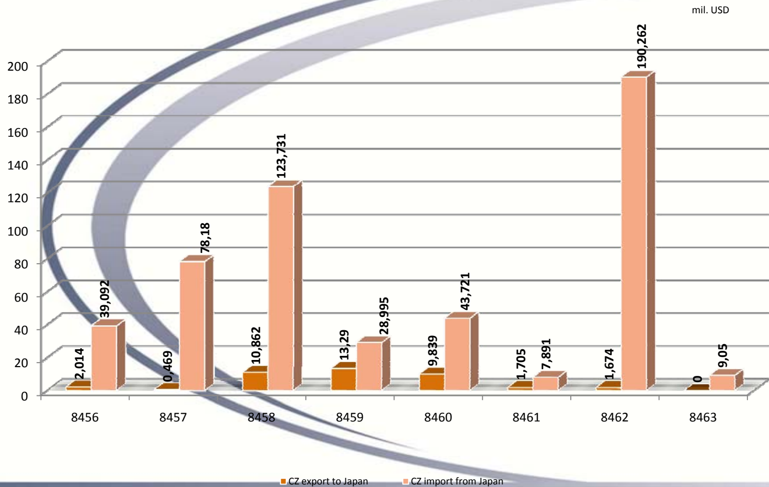
Comparison of export and import of metal cutting and metal forming machines CZ – Japan in 1999 - 2009
